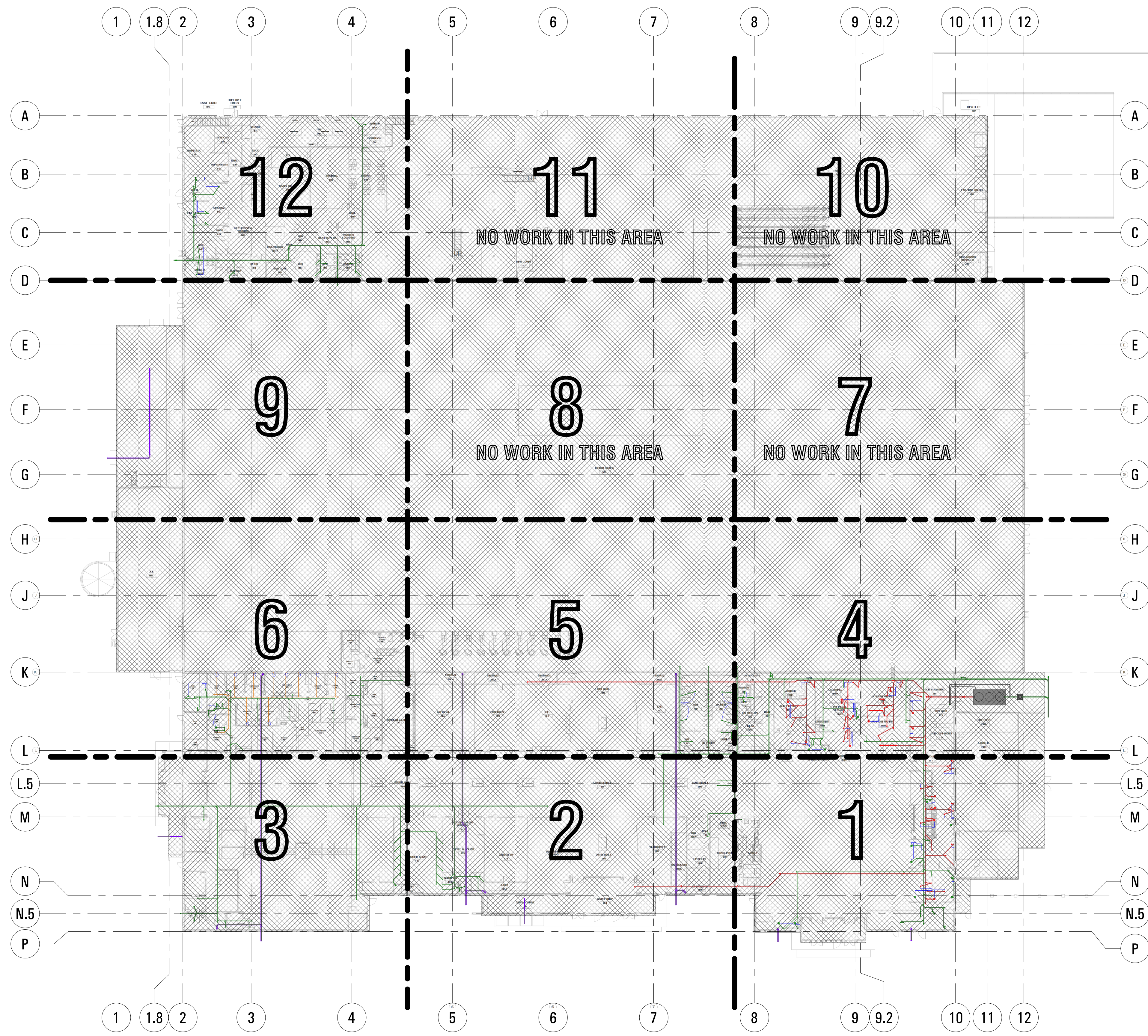
1 OVERALL PLAN 1/32" = 1'-0"
