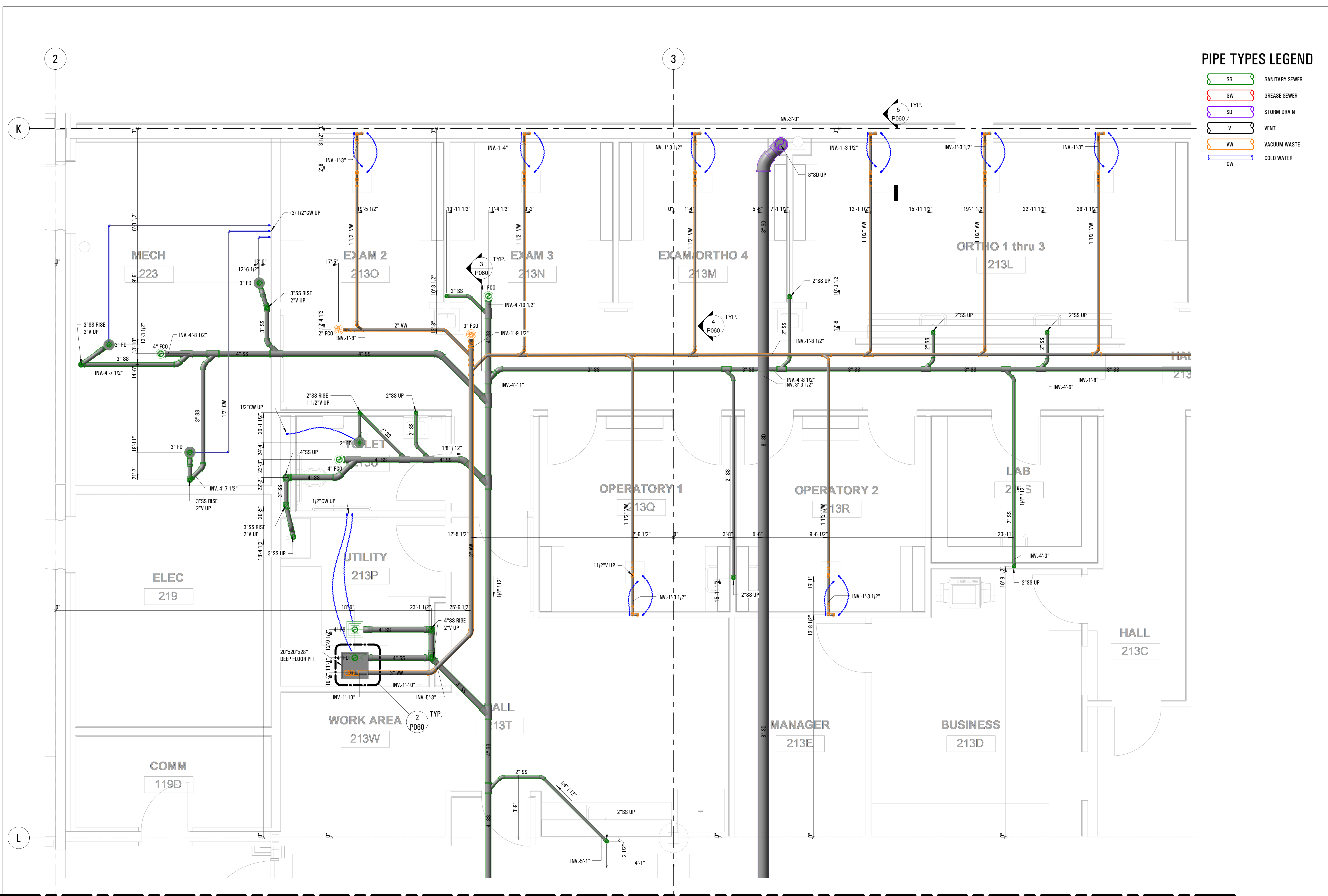
1 FLOOR PLAN 6 - Callout 1 3/8" = 1'-0"
