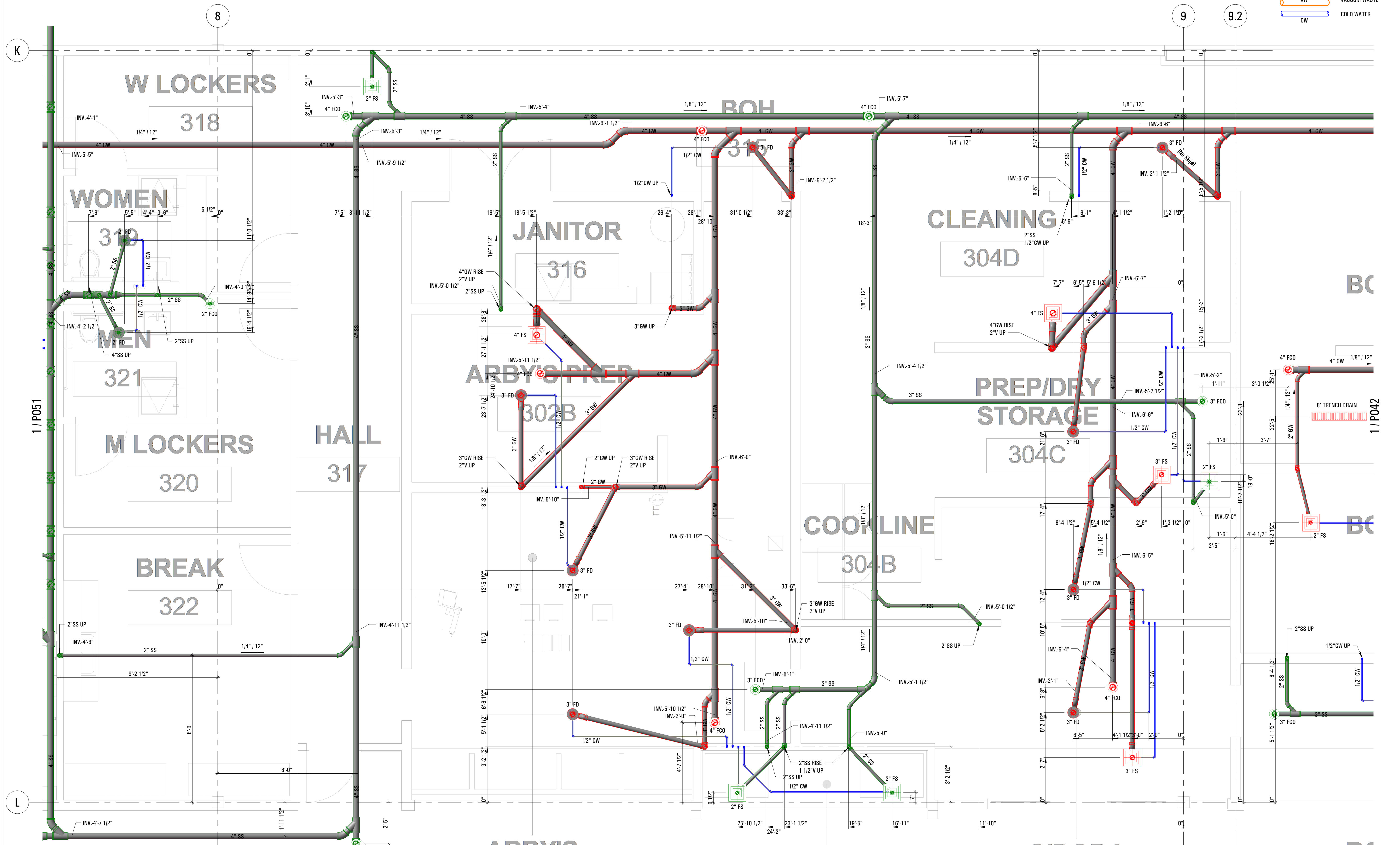
1 FLOOR PLAN 4 - Callout 1 3/8" = 1'-0"
