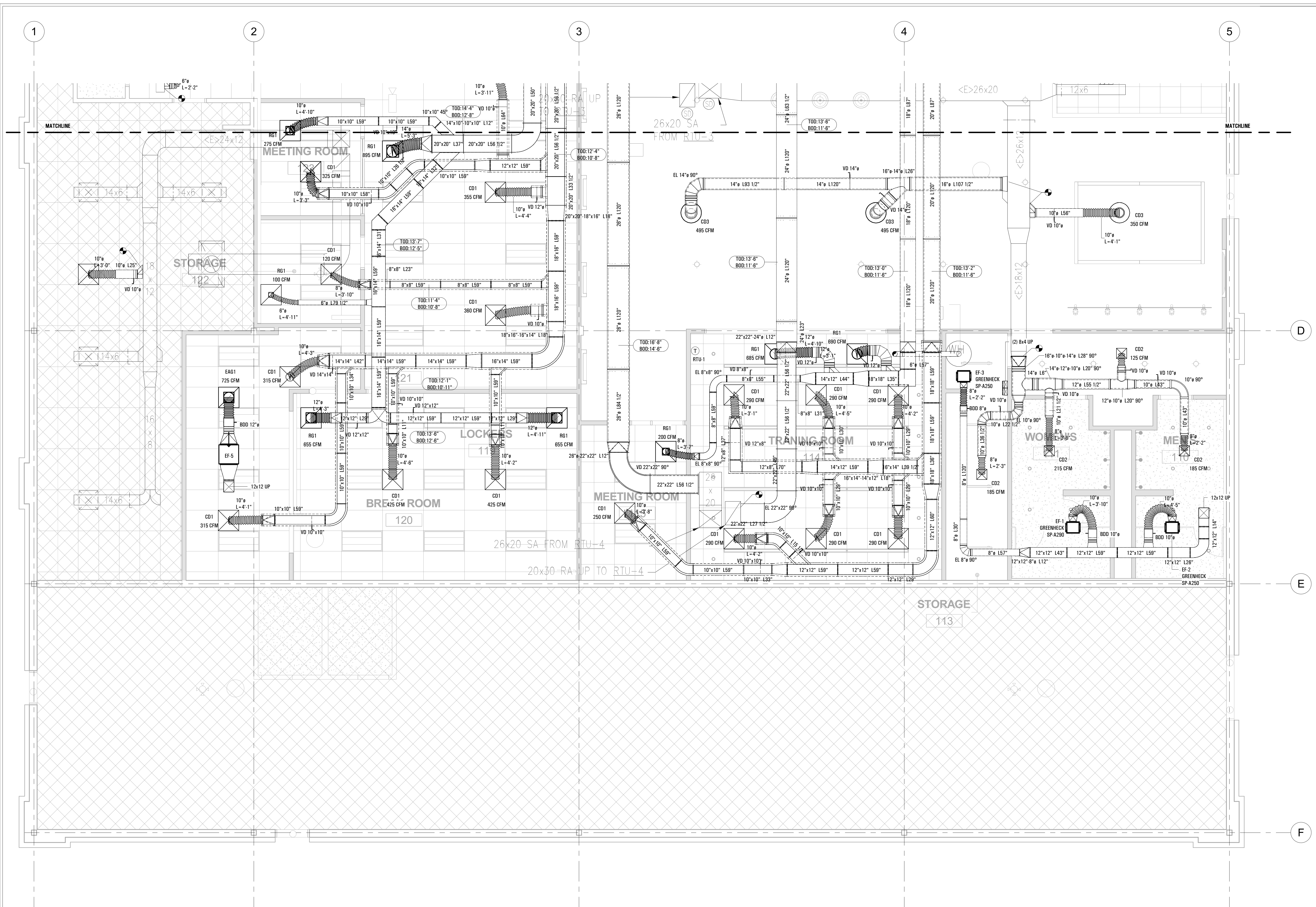
1 FIRST FLOOR - B 1/4" = 1'-0"
